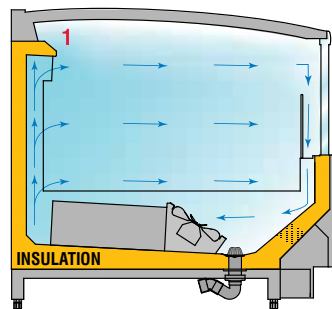
1 Cover – G: Closed w/Sliding Glass Door
